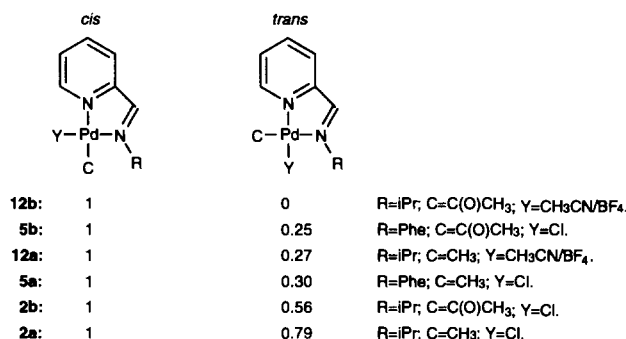
Fig. 8. cis : trans ratios of 2a , 2b , 5a , 5b , 12a and 12b .
