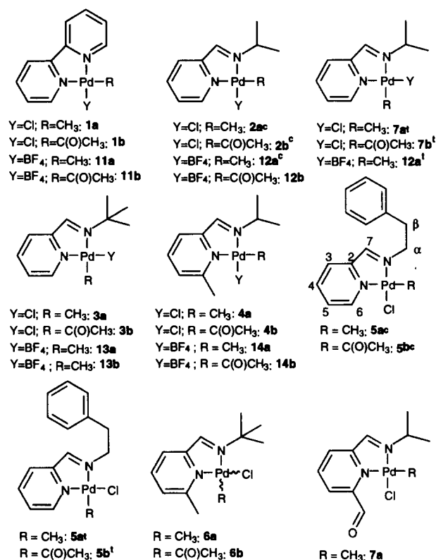
Fig. 2. Structure and numbering of the methyl- and acetyl-palladium compounds 1a–14a and 1b–14b . The adopted numbering scheme of the R-PyCa ligands 2–7 is shown only for 5 . The superscript t indicates a trans configuration, and the superscript c a cis configuration of the methyl and the imino nitrogen.
